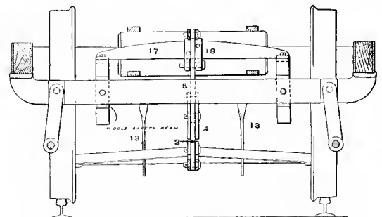
Fig. 1542. Transverse Section.
